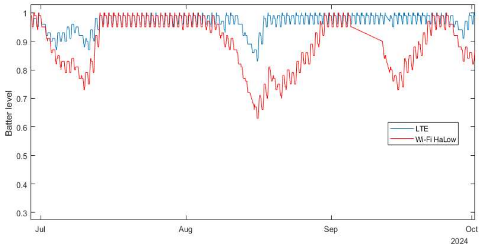
Figure 8 The devices batter level varition with different communication methods.
