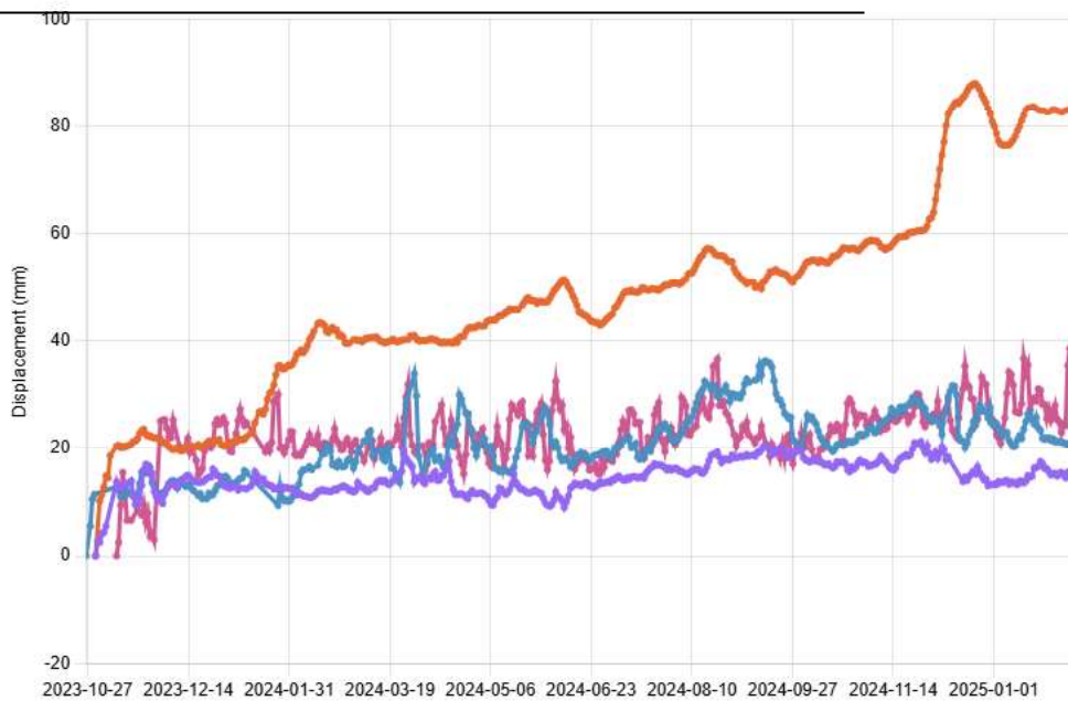
Figure 11 3D displacement of 4 monitoring nodes in Site 2.
